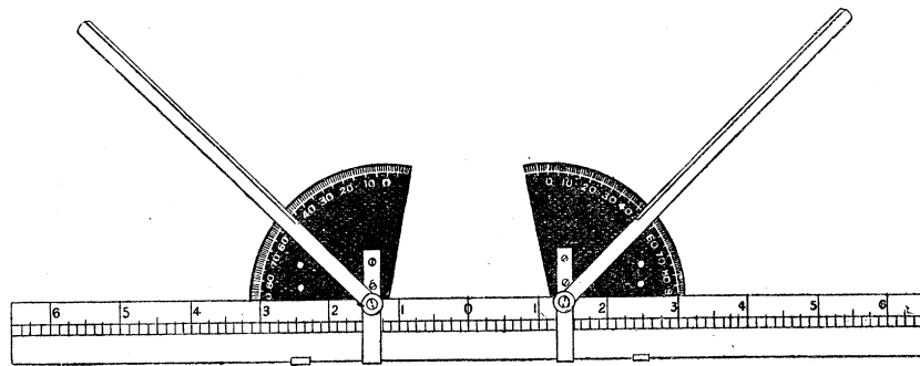
GONIOMETER \frac{1}{3} natural size
